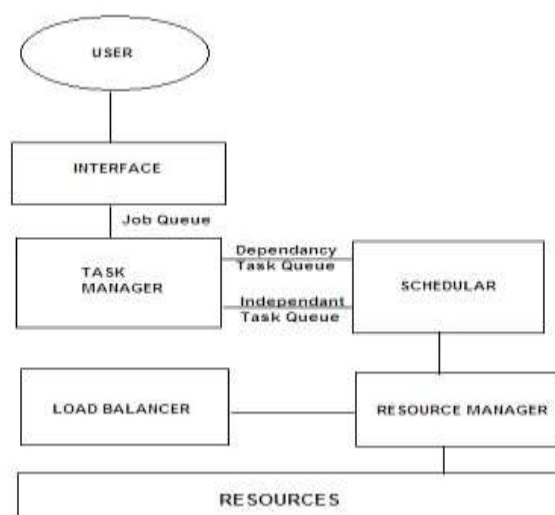
Figure 6: Scheduling and load balancing design.
