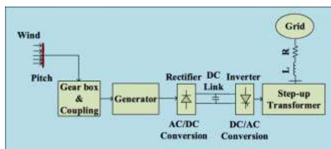
Fig. 2 Wind Energy Generation Process
