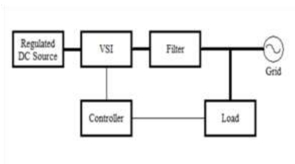
Fig. 1 Block diagram of solar and wind connected grid.
