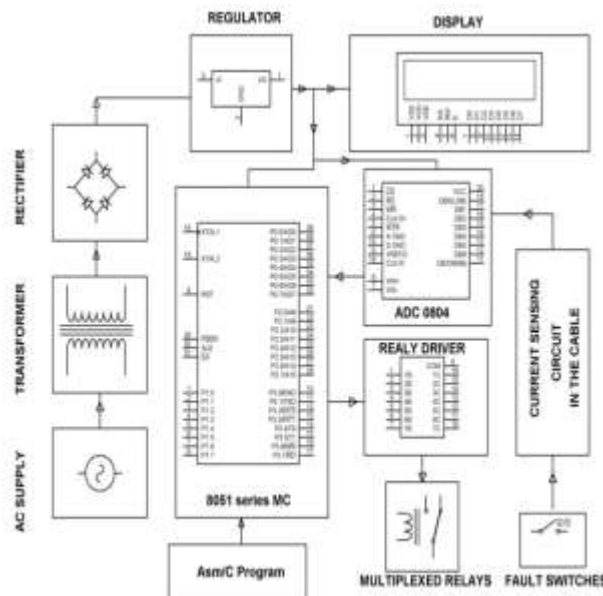
Fig1 : Block Diagram of Under ground Cable Fault Distance Locator.
