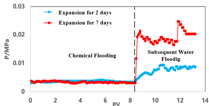
Fig.7 Expansion of MDS in porous media
