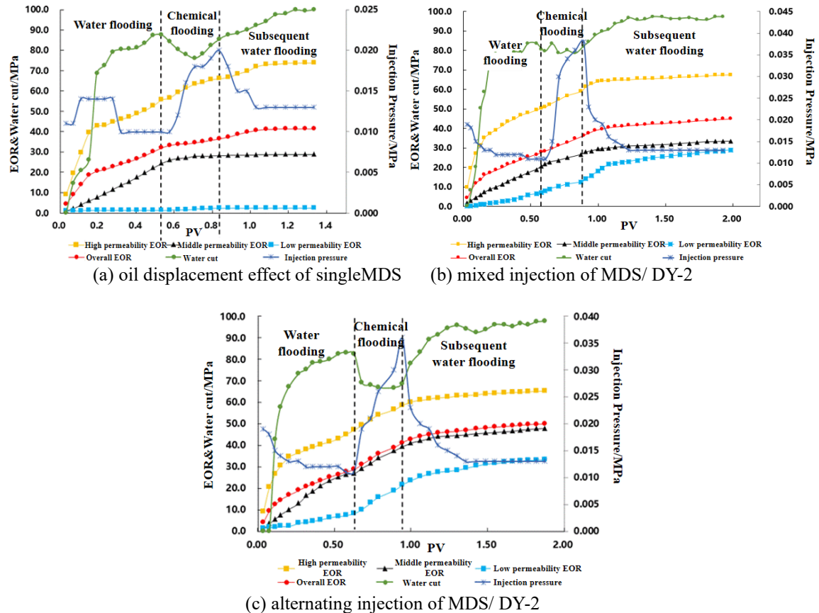
Fig.8 Dynamic characteristic curve of injection mode optimization
