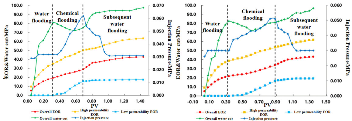
(a) 2000 mg/L DY-2 polymer and 3000 mg/L MDS (b) 1000 mg/L DY-2 polymer and 4000 mg/L MDS Fig.10 Dynamic characteristic curve of composition and concentration optimization
