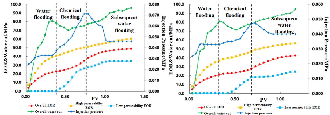
(a) the ratio of polymer to MDS is 2:1 (b) the ratio of polymer to MDS is 1:2
