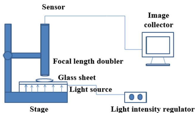
Fig.2 Particle size experimental process of MDS
