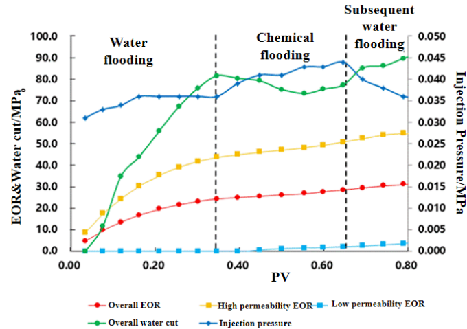
Fig.9 Single MDS oil displacement effect
