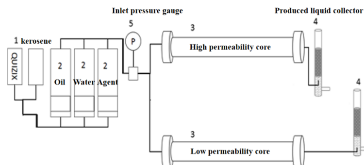
Fig.3 Physical simulation experiment equipment
