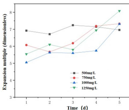
Fig.5 Hydration expansion of MDS /dy-2 solution
