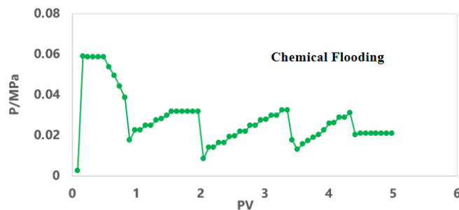
Fig.6 MDS injectability in the reservoir environment
