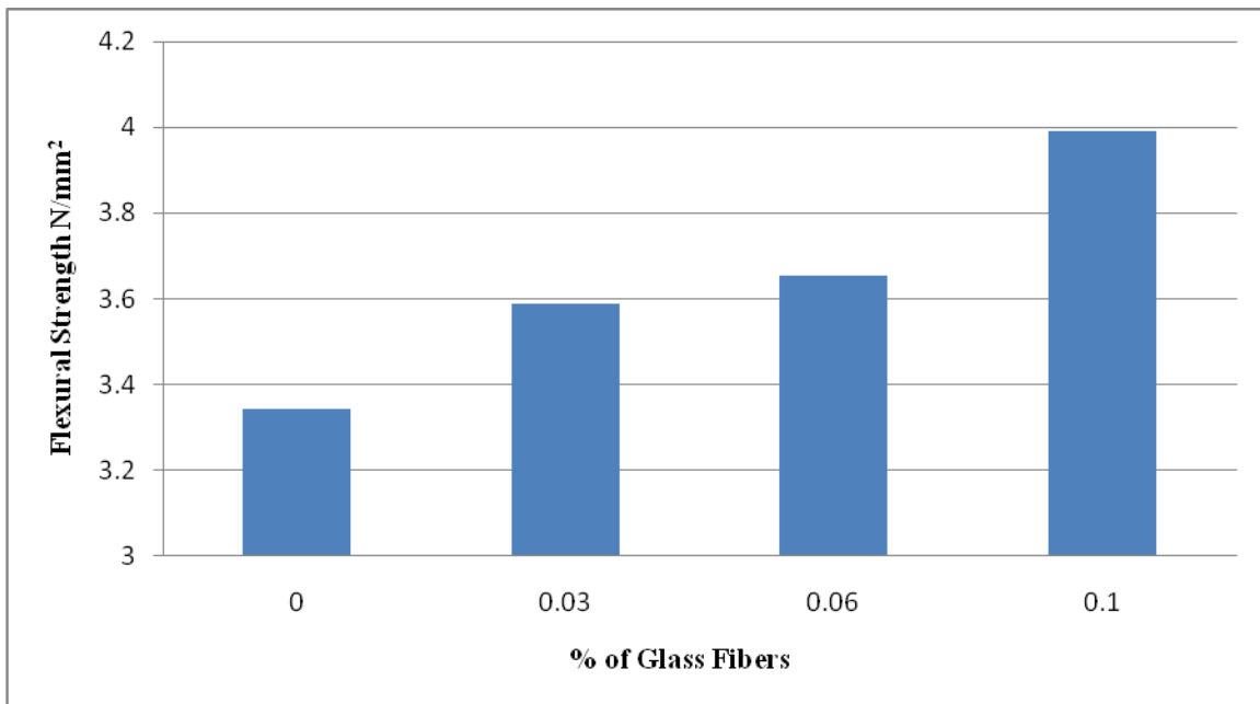
Fig. 2 Flexural strength of % of Glass Fiber
