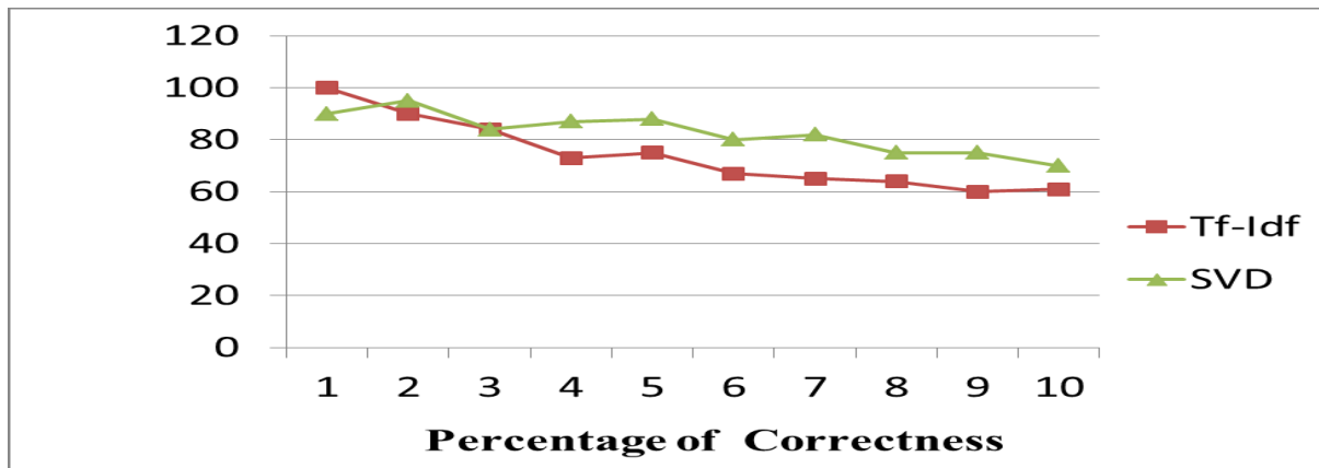
Performance comparison graph between SVD and TF-IDF
