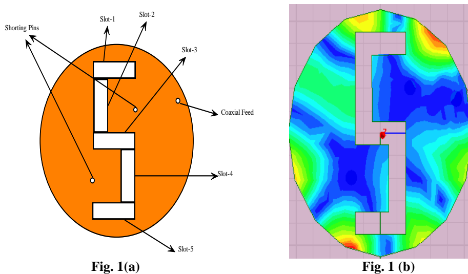
Figure 1. The geometry (a), and current distribution using HFSS simulation software of proposed S-shaped circular patch antenna (b).
