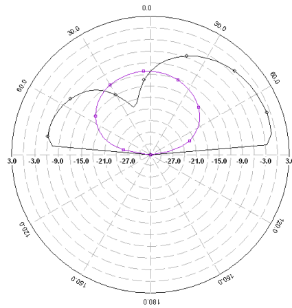
Fig. 7 (a) Radiation Pattern at 2.63 GHz
