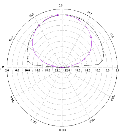
Fig. 7 (b) Radiation Pattern at 3.12 GHz
