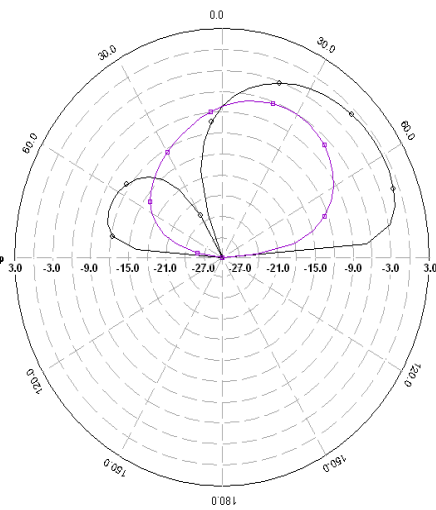
Fig. 7(d) Radiation Pattern at 6.3 GHz
