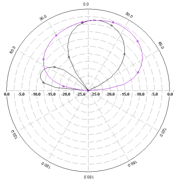
Fig. 7(e) Radiation Pattern at 8.23 Ghz
