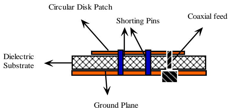
Figure 2: Side view of proposed antenna
