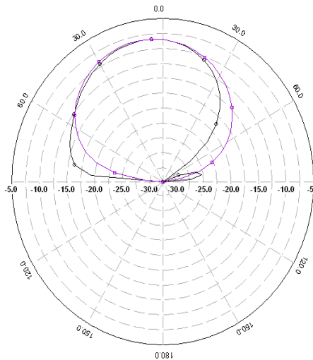
Fig. 7(c) Radiation Pattern at 4.79 GHz
