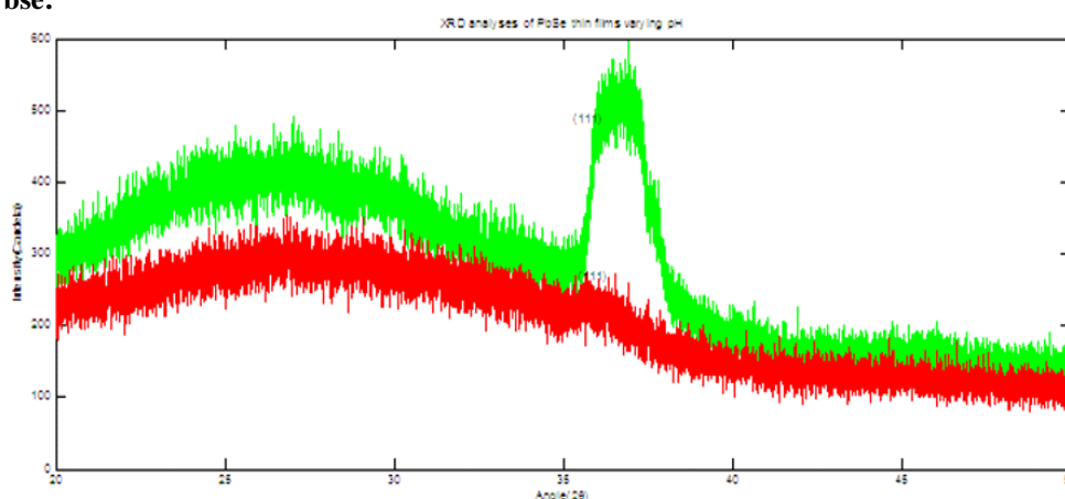
FIGURE:2 XRD OF 2ml (Green) And 4ml (Red) Pbse Thin Films
