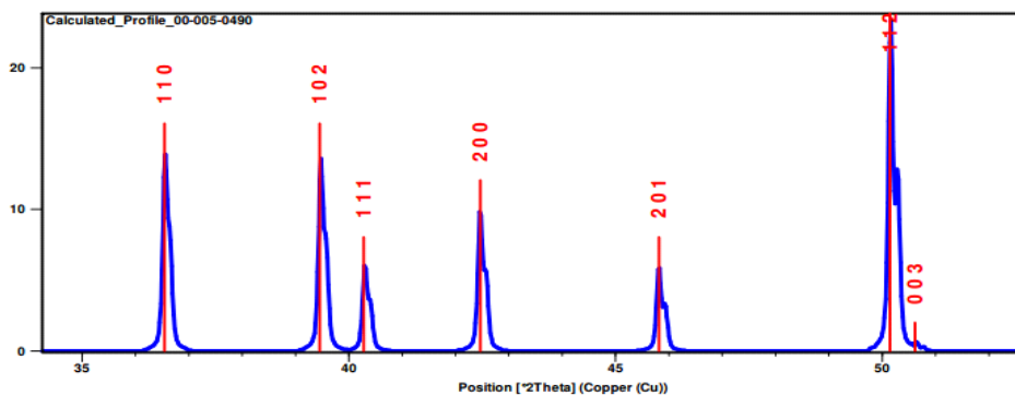
FIGURE: 1 Diffraction Peaks Of Cu
