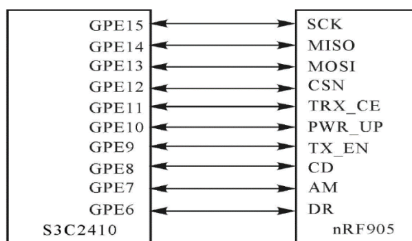
Fig. 4 Diagram of connection between S3C2410 and nRF905
