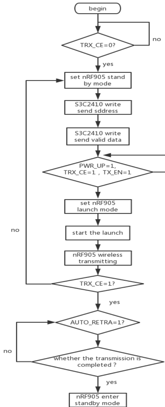
Fig. 5 Wireless transmission flow chart
