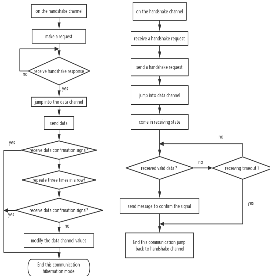
Fig. 7 Frequency hopping communication flow chart
