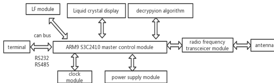
Fig. 3 On-vehicle PKE overall block diagram
