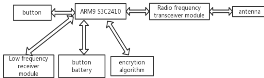
Fig. 2 PKE "key" overall block diagram
