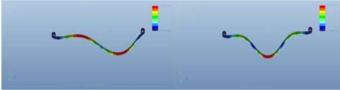
Fig. 3: Mode Shape 2
