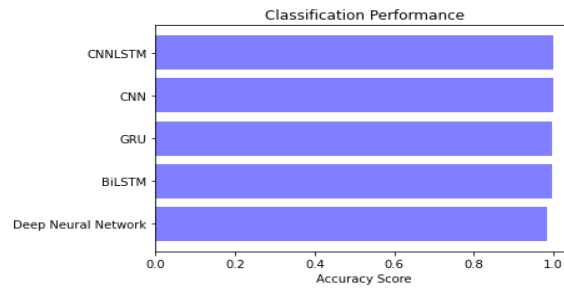
Fig 10 Accuracy graph
