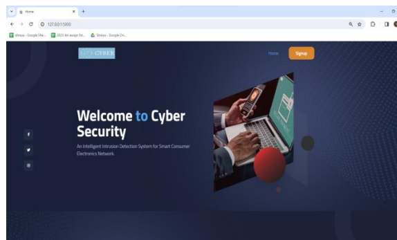
Fig 13 Home page
